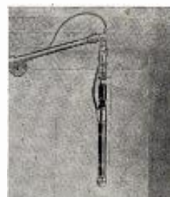
Shows TV 655 suspended on a boom. Omnidirectional polar pattern and firm swivel permits easy, diverse use.
